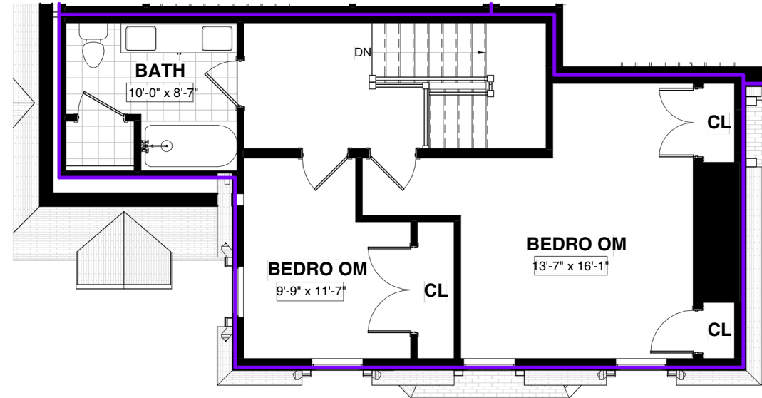
Third floor
